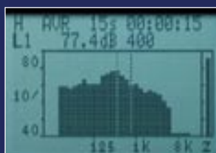
▶ Third octave band spectrum ("third octave" option)
